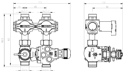
DN 15SF HF
