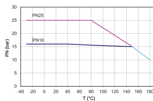
Diagram PN-T (pressure-temperature) Diagram PN-T (pressure-temperature)
