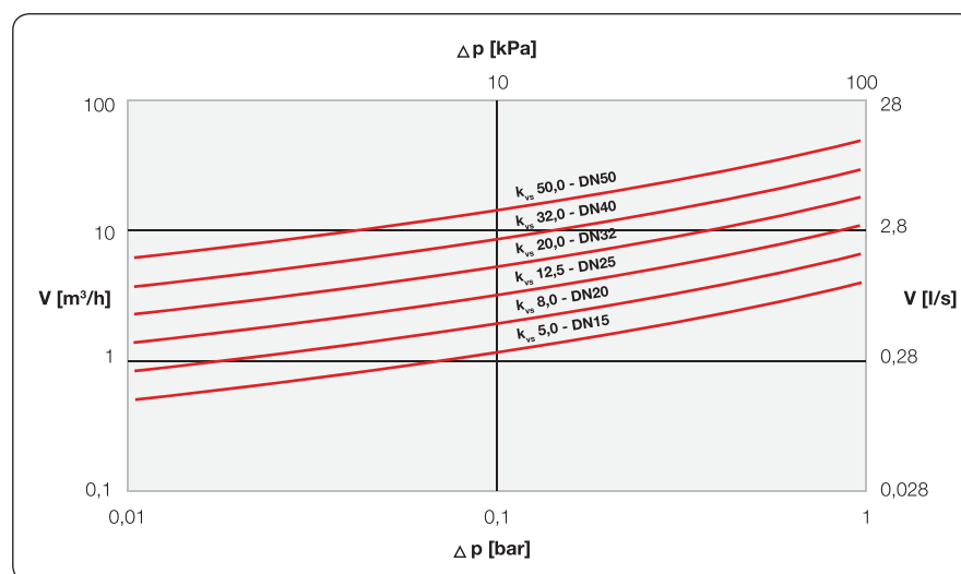
Flow Diagram
