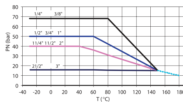
Diagram PN-T (pressure-temperature) Diagram PN-T (pressure-temperature)
